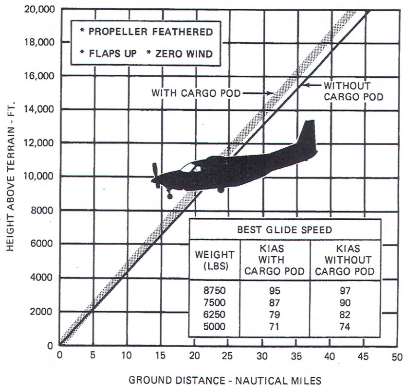
Figure 3-1. Maximum Glide
